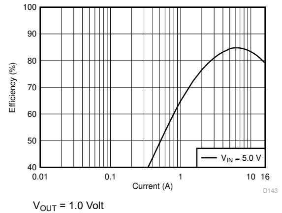
图 8-3. Efficiency in Forced-PWM-Four-Phase Mode
