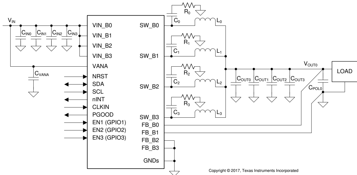
图 8-1. 4-Phase Configuration
