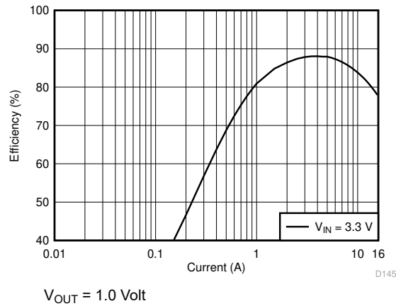
图 8-2. Efficiency in Forced-PWM-Four-Phase Mode
