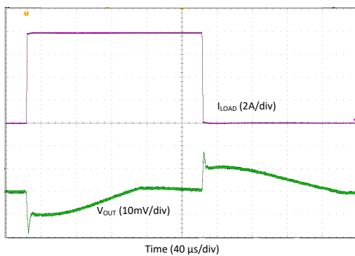
图 8-10. Output Voltage Ripple, Forced-PWM-Four-Phase Mode
