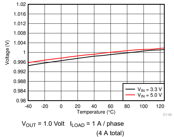
图 8-5. Output Voltage vs Temperature
