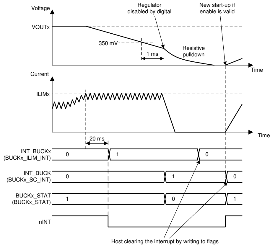
图 7-10. Overload Situation
