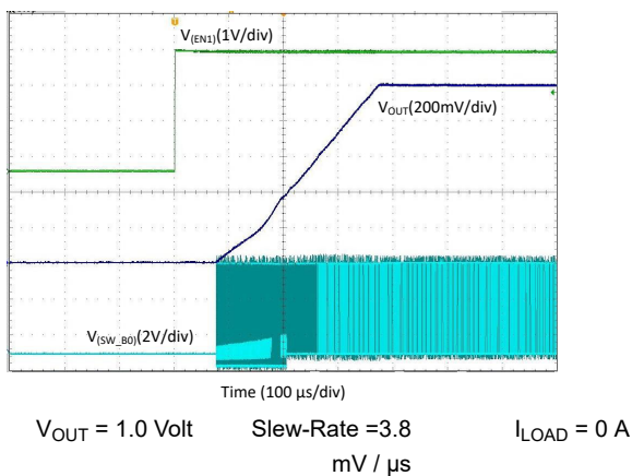
图 8-6. Start-Up With EN1, Forced-PWM-Four-Phase Mode
