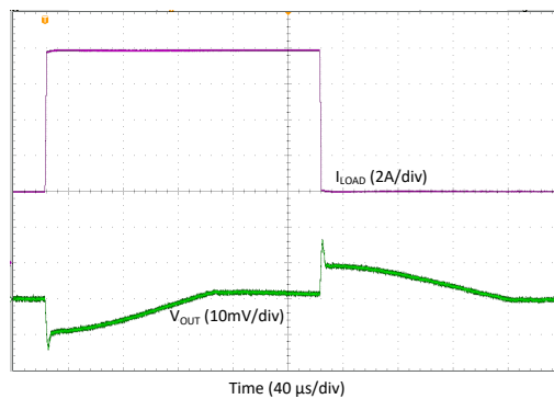
图 8-15. Transient Load Step Response, Forced-PWM-Four-Phase Mode, T_A=-40^\circ\text{C}
