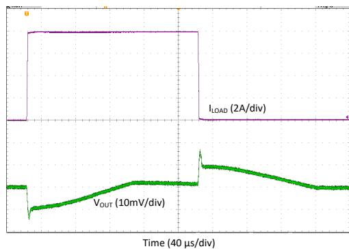
图 8-14. Transient Load Step Response, Forced-PWM-Four-Phase Mode, T_A=+25^\circ\text{C}
