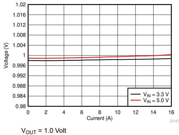
图 8-4. Output Voltage vs Load Current in Forced-PWM-Four-Phase Mode
