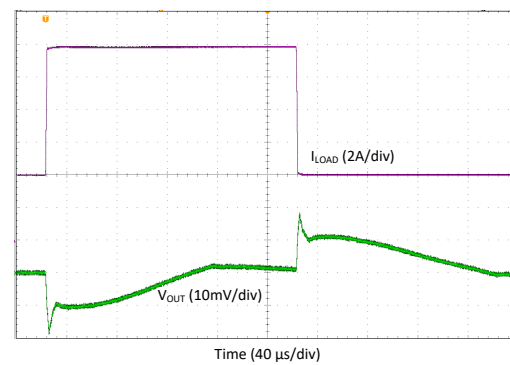
图 8-11. Transient Load Step Response, Forced-PWM-Four-Phase Mode, T_A = +25^\circ\text{C}
