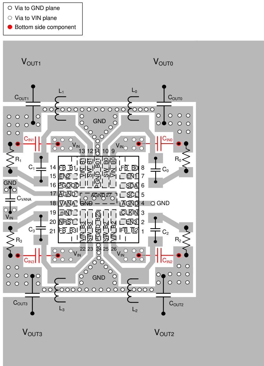
图 10-1. Board Layout
