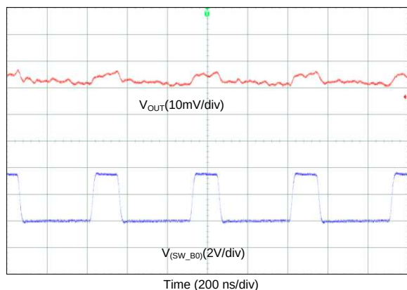
图 82. Output Voltage Ripple, Forced-PWM Mode (3-Phase Output)
