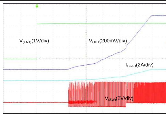
图 71. Start-Up With EN1, Forced PWM (2-Phase Output)
