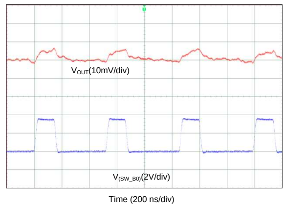
图 84. Output Voltage Ripple, Forced-PWM Mode (1-Phase Output)
