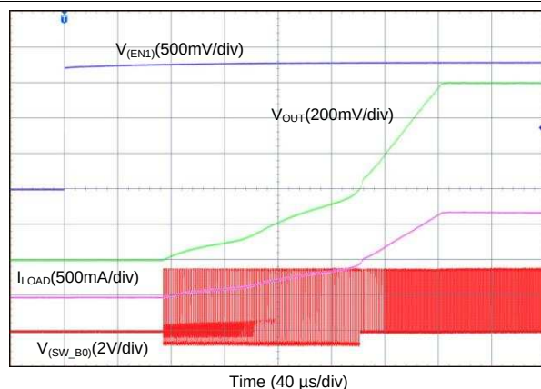
图 72. Start-Up With EN1, Forced PWM (1-Phase Output)
