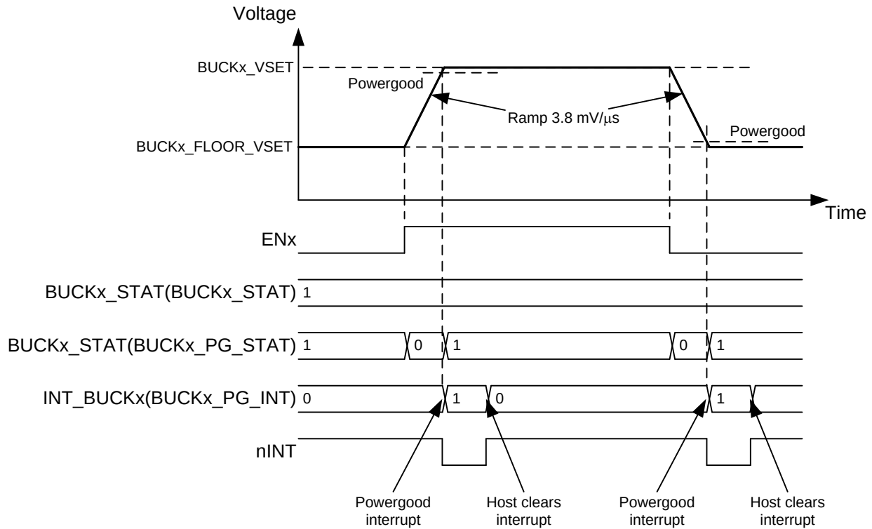
图 9. Regulator Output Voltage Change With ENx pin
