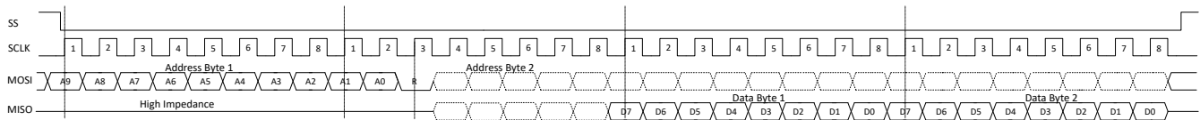
图 7-18. SPI Read Timing
