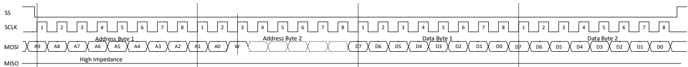
图 7-17. SPI Write Timing
