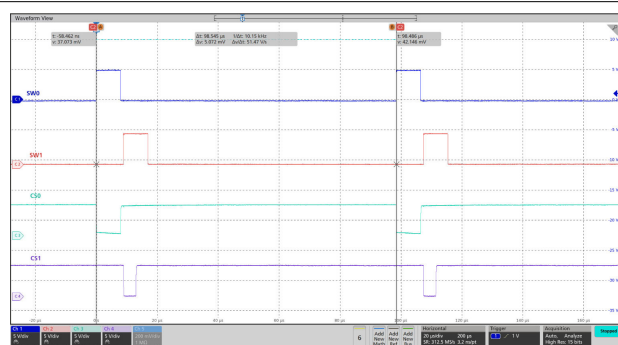
图 8-3. Scan Lines and Current Sinks Waveforms of SW0, SW1, CS0, CS1
