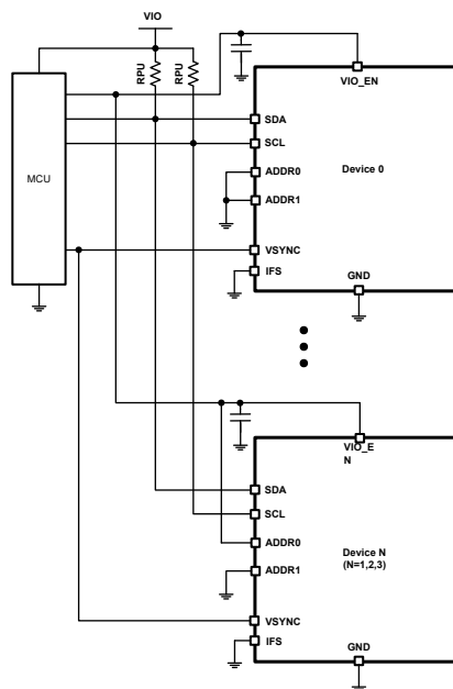
图 7-16. I²C Multiple Devices Connection
