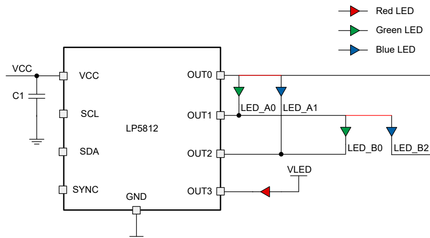
图 7-9. 混合驱动模式，2 次扫描 ( \text{led\_mode} = 6\text{h} , \text{scan\_order}_0 = 0\text{h} , \text{scan\_order}_1 = 1\text{h} , \text{mix\_sel\_led} = 8\text{h} )
