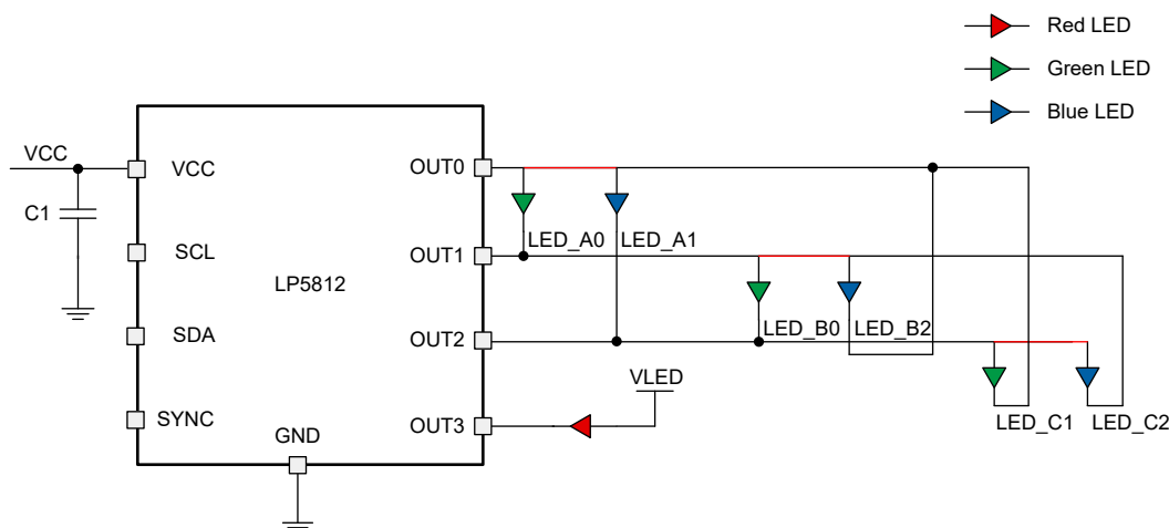
图 7-10. 混合驱动模式，3 次扫描 ( \text{led\_mode} = 7\text{h} , \text{scan\_order}_0 = 0\text{h} , \text{scan\_order}_1 = 1\text{h} , \text{scan\_order}_2 = 2\text{h} , \text{mix\_sel\_led} = 8\text{h} )
