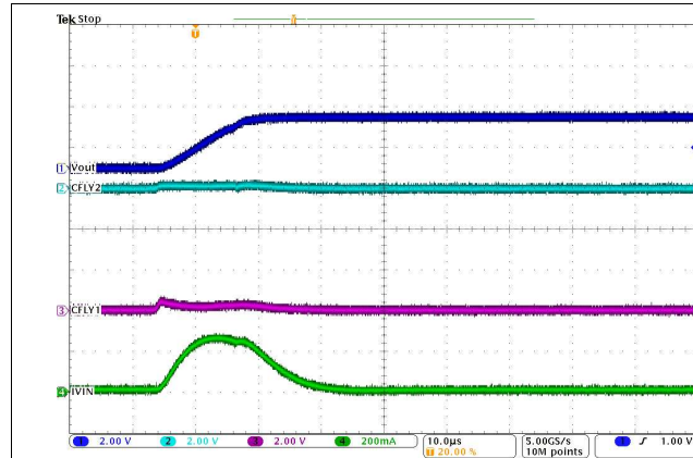
图 120. Start-Up Waveform
