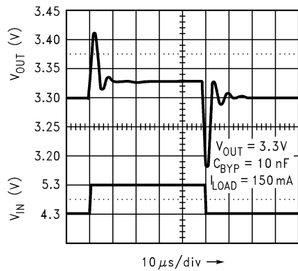
图 7-18. Line Transient Response (Legacy Chip)
