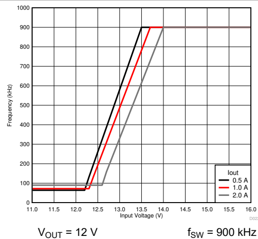
图 7-7. Frequency Foldback
