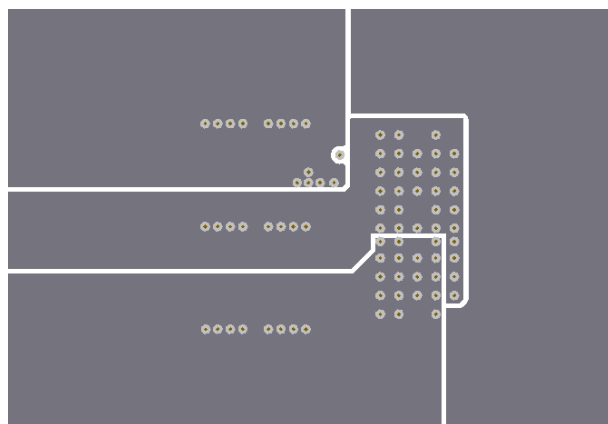
图 9-3. Typical Layer 3 Layout
