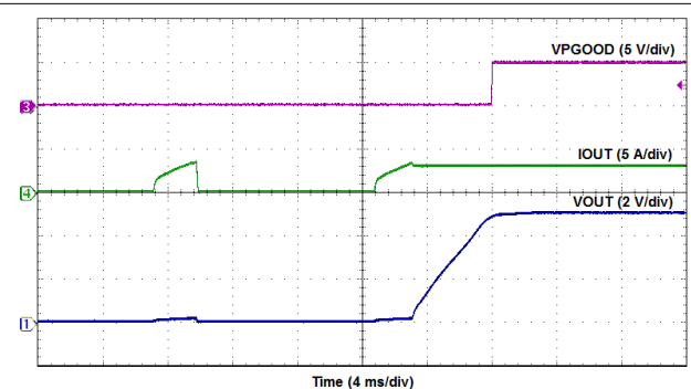
图 7-16. Removal of Overcurrent
