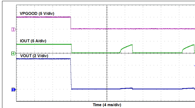
图 7-15. Overcurrent Limiting
