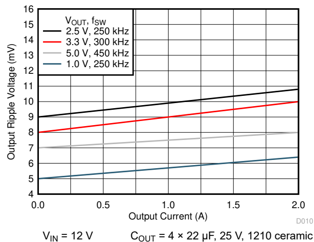
图 6-7. Voltage Ripple vs Output Current
