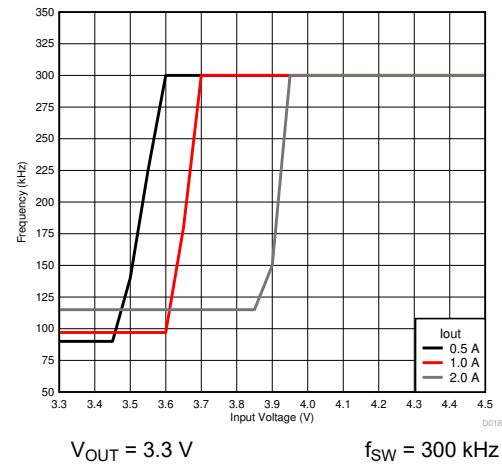
图 7-3. Frequency Foldback
