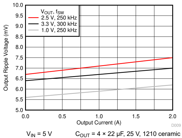
图 6-3. Voltage Ripple vs Output Current
