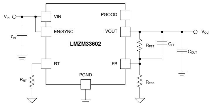
图 8-1. LMZM33602 Typical Schematic
