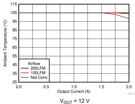
图 6-13. Safe Operating Area
