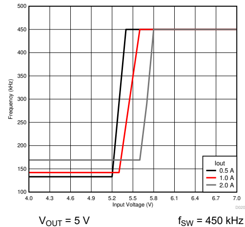
图 7-5. Frequency Foldback
