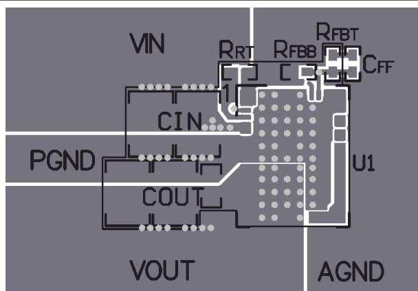
图 9-1. Typical Top-Layer Layout
