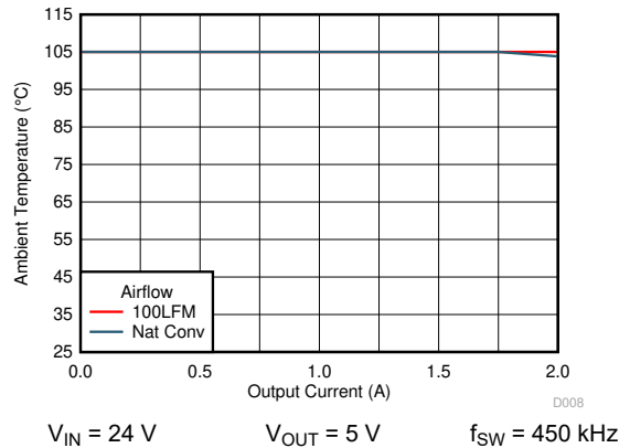
图 6-12. Safe Operating Area
