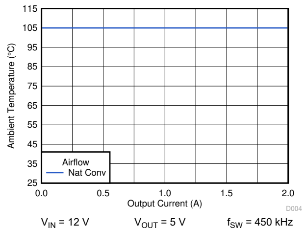
图 6-8. Safe Operating Area
