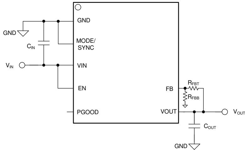
图 9-4. Adjustable 1.2-V to 15-V Output Typical Application Circuit
