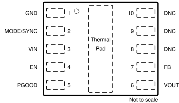
图 6-1. SIL 10-Pin MicroSiP™ Package Top View
