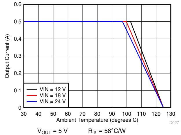
图 7-20. Ambient Temperature vs Output Current
