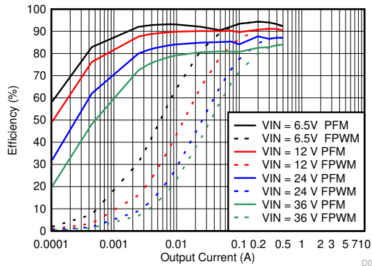
图 9-42. Efficiency for V_{OUT} = 5\text{ V}
