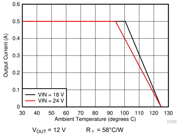
图 7-21. Ambient Temperature vs Output Current
