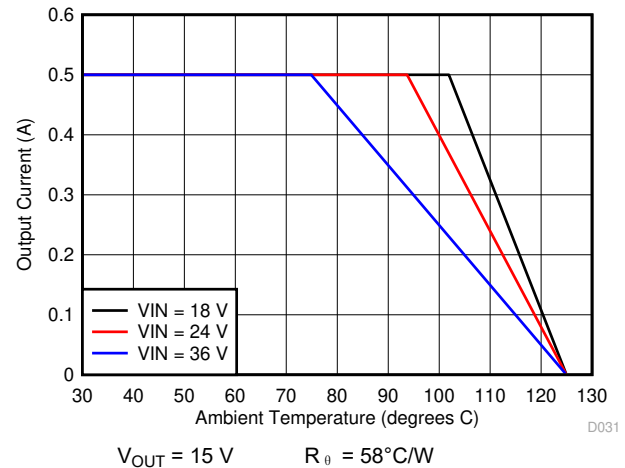
图 7-22. Ambient Temperature vs Output Current
