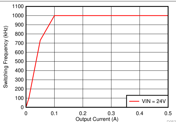
图 7-26. Auto PFM Mode Switching Frequency vs Output Current
