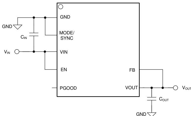
图 9-1. Fixed 5-V or 3.3-V Typical Application Circuit
