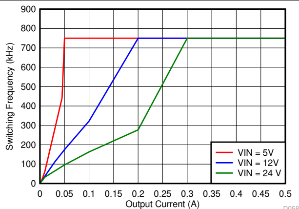
图 7-25. Auto PFM Mode Switching Frequency vs Output Current
