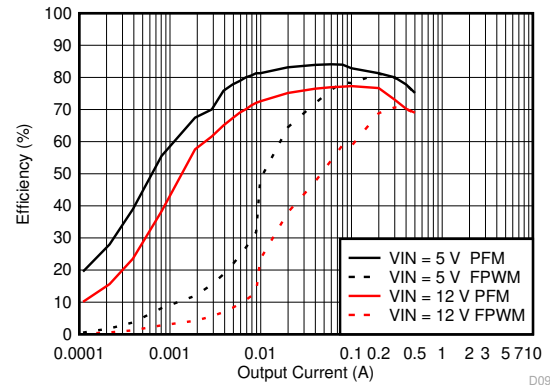
图 9-37. Efficiency for V_{OUT} = 1.2\text{ V}
