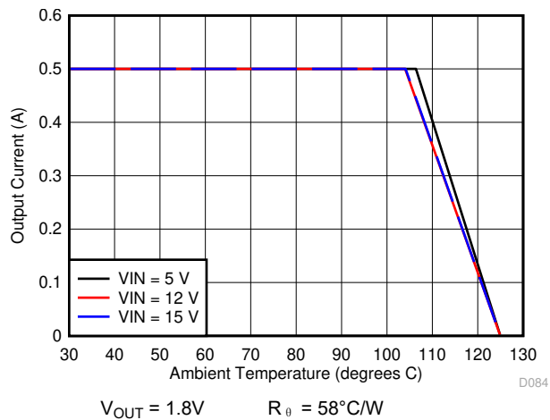
图 7-17. Ambient Temperature vs Output Current
