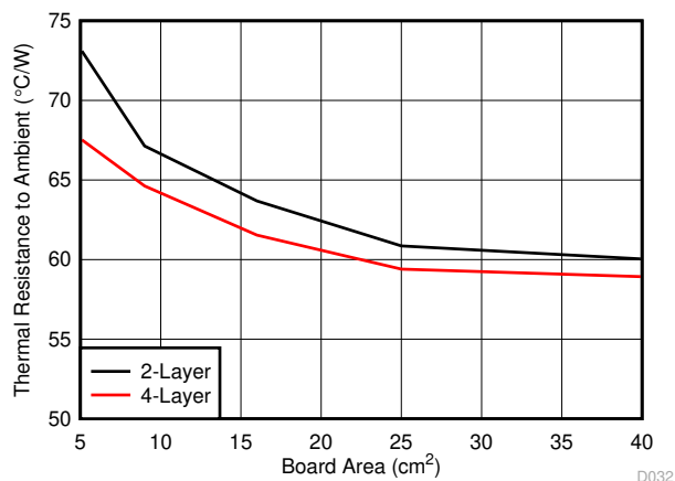
图 9-48. Package Thermal Resistance vs Board Copper Area
