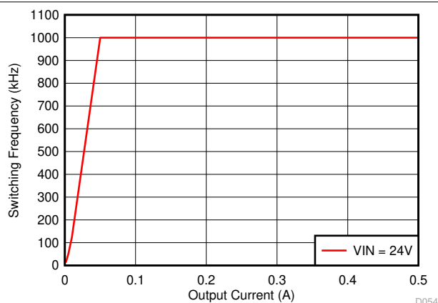
图 7-27. Auto PFM Mode Switching Frequency vs Output Current
