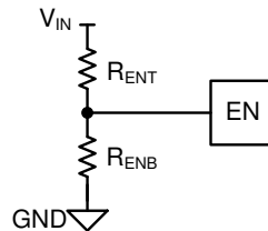
图 9-5. Enable Divider to Set External UVLO Threshold
