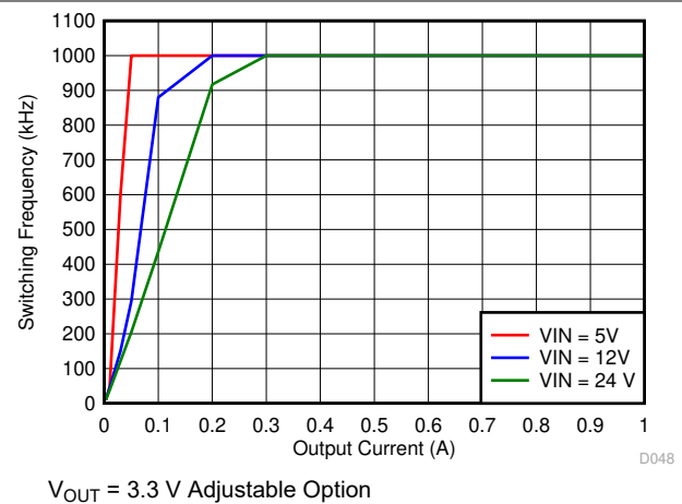
图 7-24. Auto PFM Mode Switching Frequency vs Output Current
