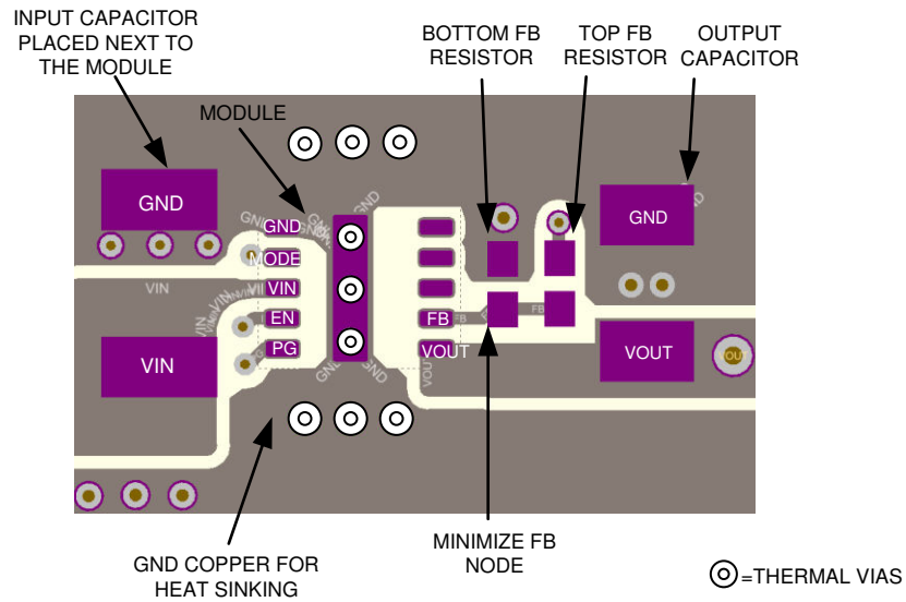
图 9-50. Layout Example With Adjustable Output Version
