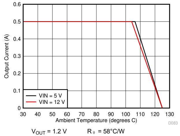
图 7-16. Ambient Temperature vs Output Current
