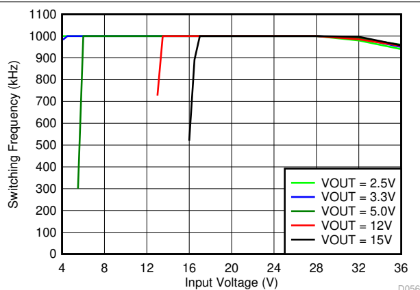
图 7-30. Switching Frequency vs Input Voltage for Adjustable Output Options at Full Load
