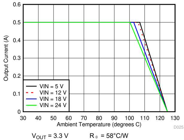
图 7-19. Ambient Temperature vs Output Current
