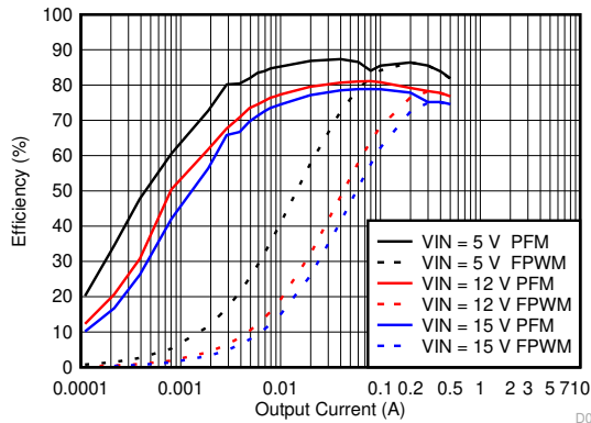
图 9-36. Efficiency for V_{OUT} = 1.8\text{ V}
