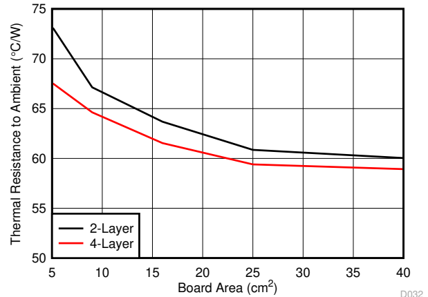
图 7-8. Package Thermal Resistance vs Board Copper Area, No Air Flow
