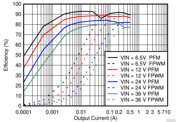
图 9-12. Efficiency
