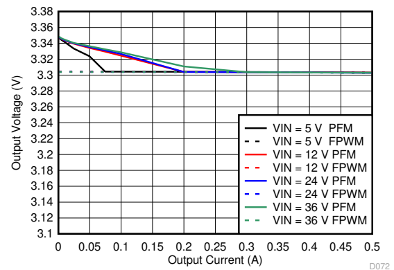
图 9-45. Line and Load Regulation for V_{OUT} = 3.3\text{ V}
