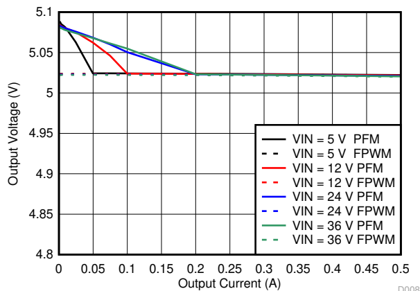
图 9-10. Line and Load Regulation
