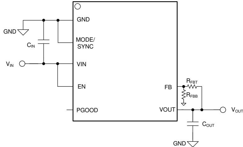
图 9-2. Adjustable 1.2-V to 15-V Output Typical Application Circuit
