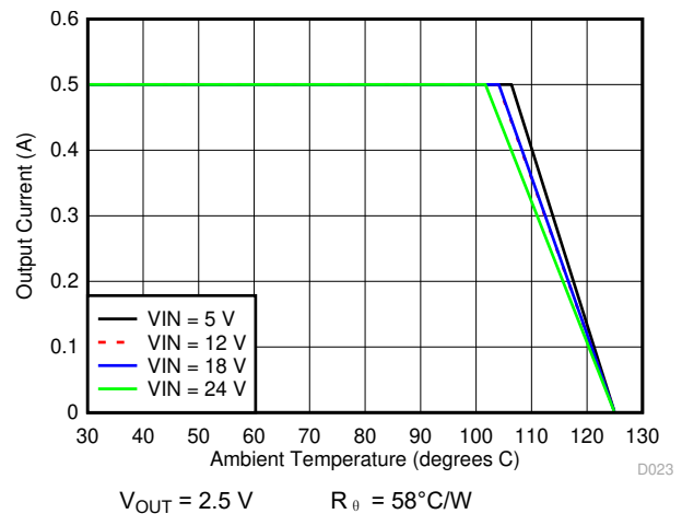
图 7-18. Ambient Temperature vs Output Current
