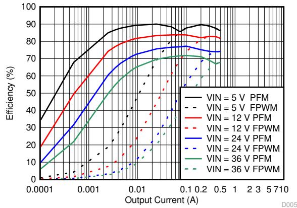
图 9-30. Efficiency
