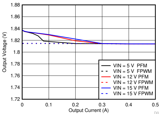
图 9-38. Line and Load Regulation for V_{OUT} = 1.8\text{ V}
