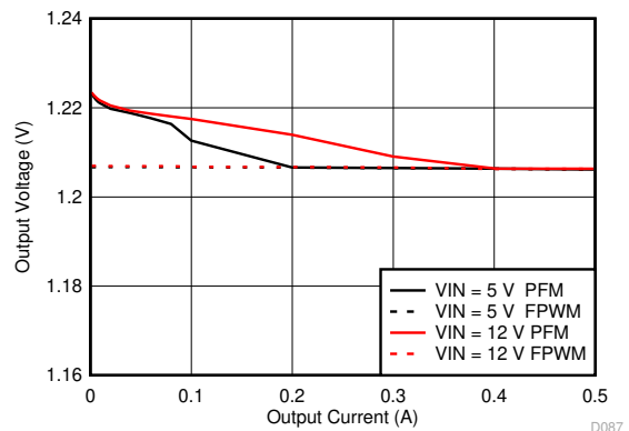
图 9-39. Line and Load Regulation for V_{OUT} = 1.2\text{ V}
