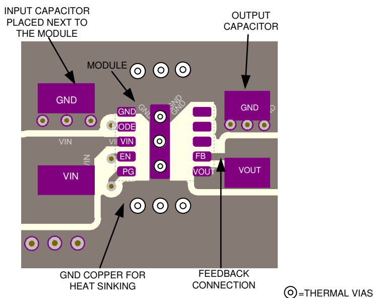
图 9-49. Layout Example With Fixed Output Version
