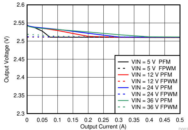
图 9-34. Line and Load Regulation
