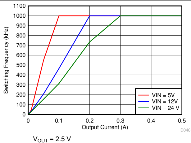
图 7-23. Auto PFM Mode Switching Frequency vs Output Current
