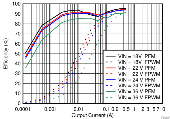
图 9-24. Efficiency
