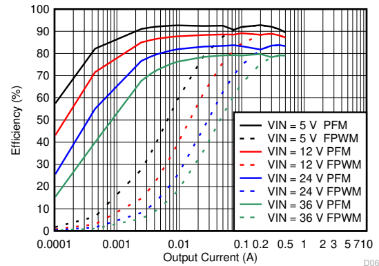
图 9-43. Efficiency for V_{OUT} = 3.3\text{ V}
