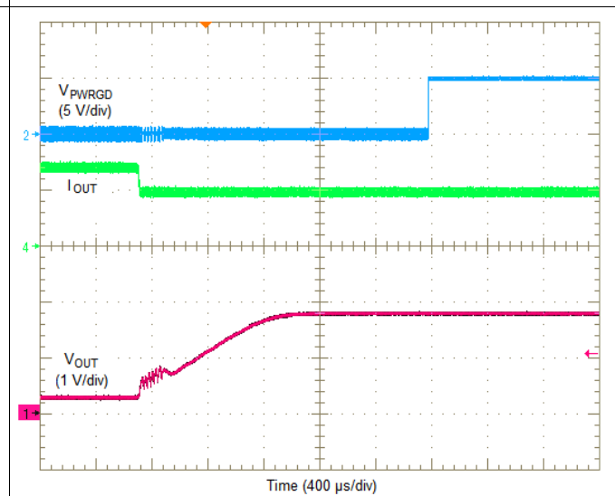
Figure 33. Removal of Overcurrent (Cycle-by-Cycle)
