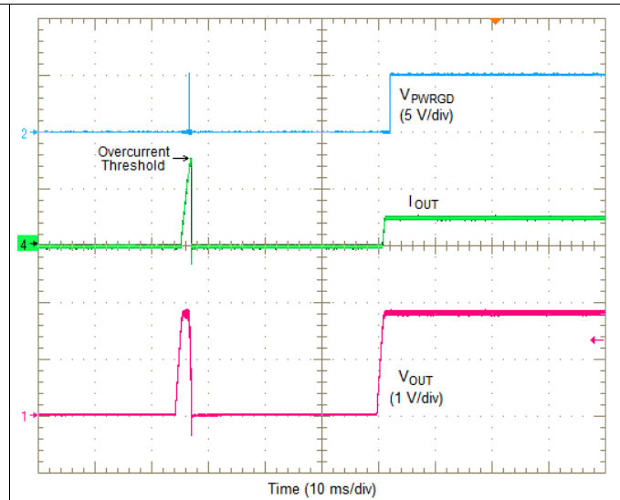
Figure 31. Removal of Overcurrent (Hiccup)
