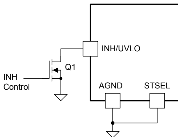
图 30. Typical Inhibit Control
