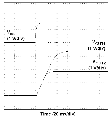
图 40. Simultaneous Tracking Waveforms
