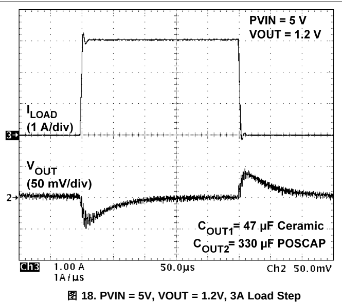
图 18. P_{VIN} = 5V , V_{OUT} = 1.2V , 3A Load Step
