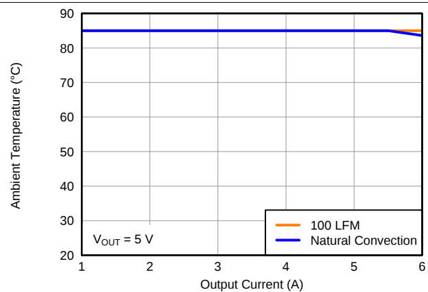
图 14. Safe Operating Area
