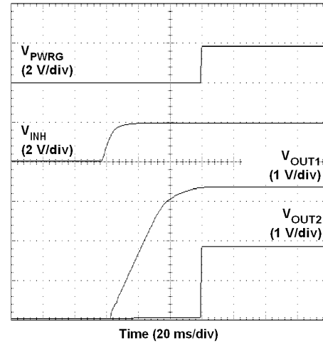
图 38. Sequencing Waveforms
