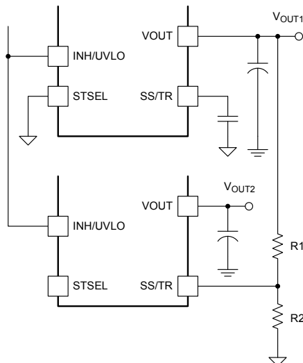
图 39. Simultaneous Tracking Schematic
