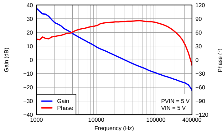
图 10. V_{OUT}=1.2\text{ V} , I_{OUT}=3\text{ A} , C_{OUT1}=47\text{ }\mu\text{F} ceramic, C_{OUT2}=330\text{ }\mu\text{F} POSCAP, f_{SW}=480\text{ kHz}
