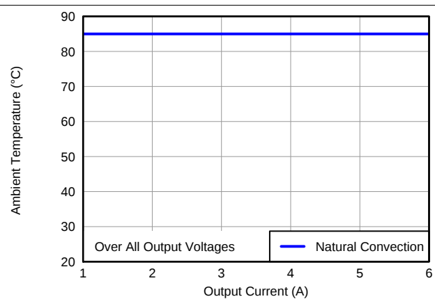
图 4. Safe Operating Area
