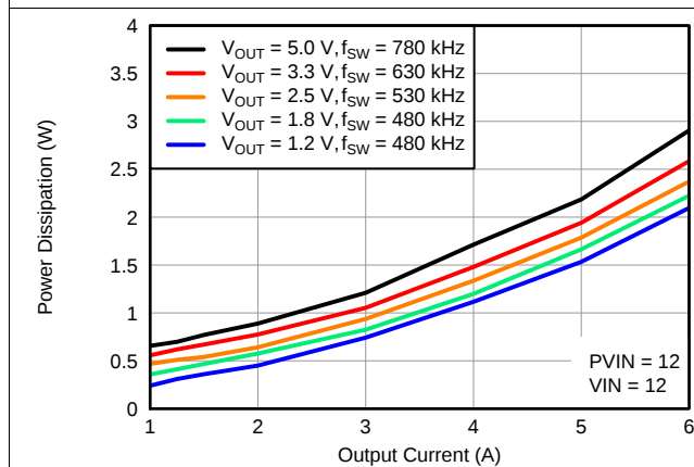
图 3. Power Dissipation vs. Output Current
