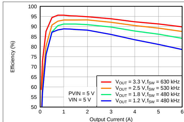
图 6. Efficiency vs. Output Current
