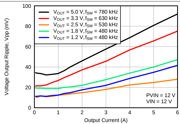
图 2. Voltage Ripple vs. Output Current
