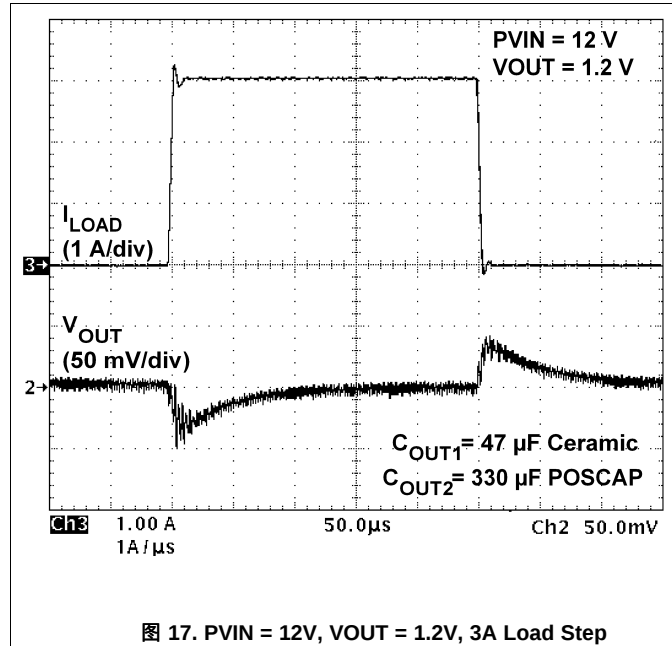
图 17. P_{VIN} = 12V , V_{OUT} = 1.2V , 3A Load Step
