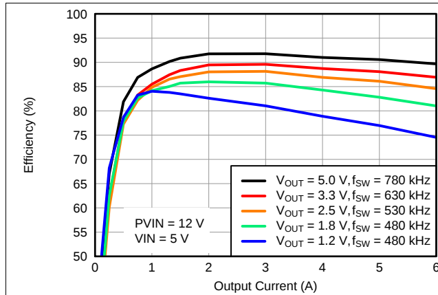
图 11. Efficiency vs. Output Current
