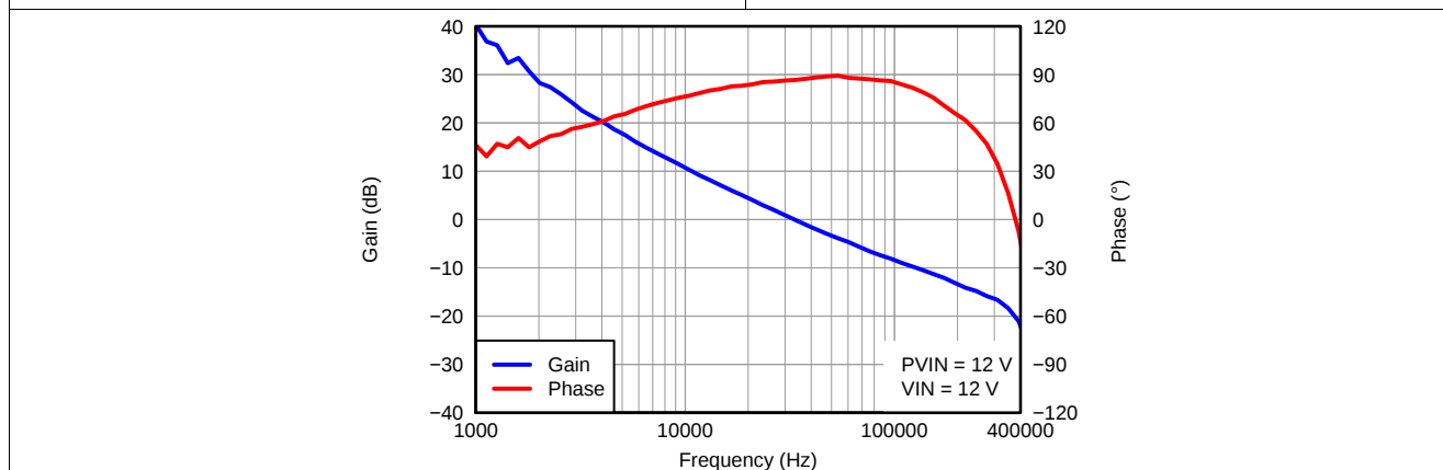
图 5. V_{OUT}=1.2\text{ V} , I_{OUT}=3\text{ A} , C_{OUT1}=47\text{ }\mu\text{F} ceramic, C_{OUT2}=330\text{ }\mu\text{F} POSCAP, f_{SW}=480\text{ kHz}
