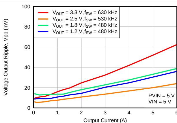
图 7. Voltage Ripple vs. Output Current
