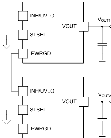
图 37. Sequencing Schematic
