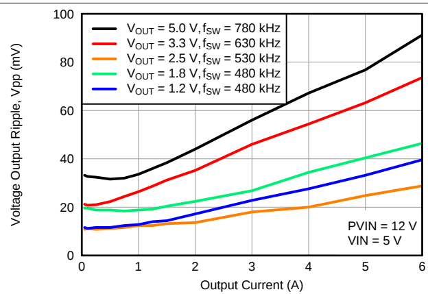
图 12. Voltage Ripple vs. Output Current
