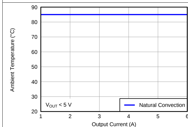
图 15. Safe Operating Area
