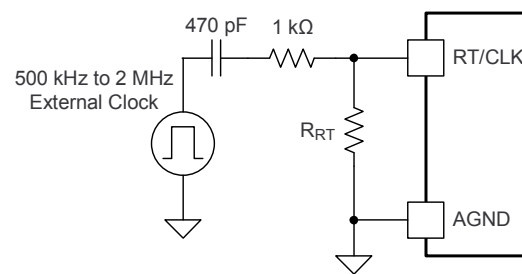
Figure 28. CLK/RT Configuration
