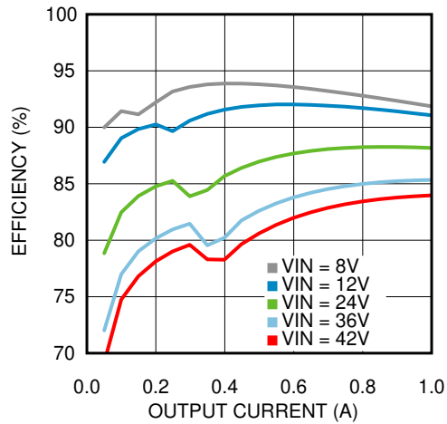
图 6-13. Efficiency V_{OUT} = 5\text{ V} , T_A = 85^\circ\text{C}
