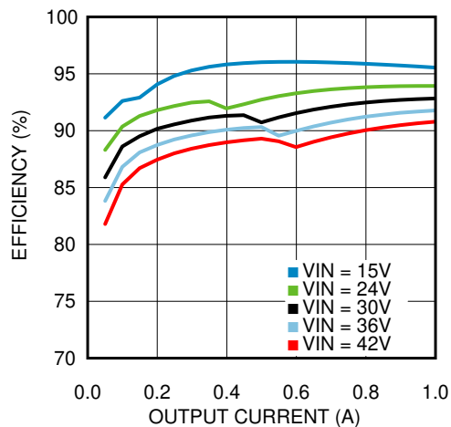
图 6-15. Efficiency V_{OUT} = 12\text{ V} , T_A = 85^\circ\text{C}
