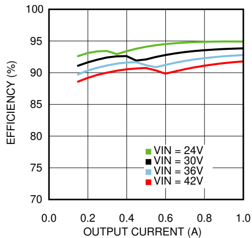
图 6-17. Efficiency V_{OUT} = 15\text{ V} , T_A = 85^\circ\text{C}
