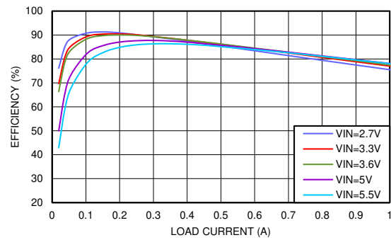
图 8-3. Efficiency V_{OUT} = 1.2\text{ V}
