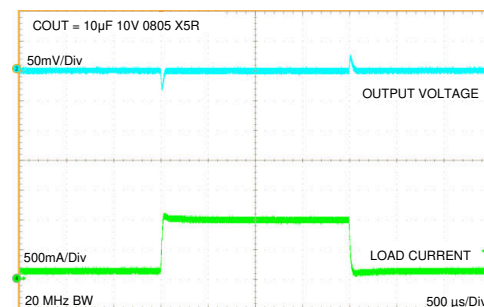
图 8-5. Load Transient V_{OUT} = 1.2\text{ V}
