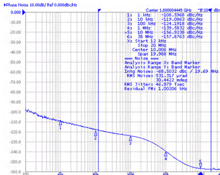
图 8-12. Typical Jitter
