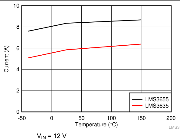
图 7-3. High-Side/Peak Current Limit for LMS36x5-Q1
