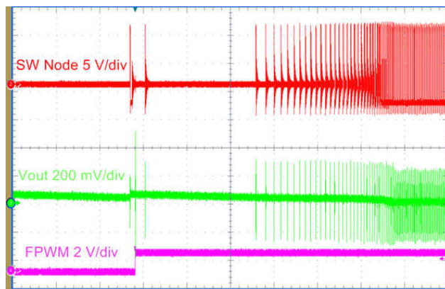
图 9-29. Mode Change Transient AUTO to FPWM mode
