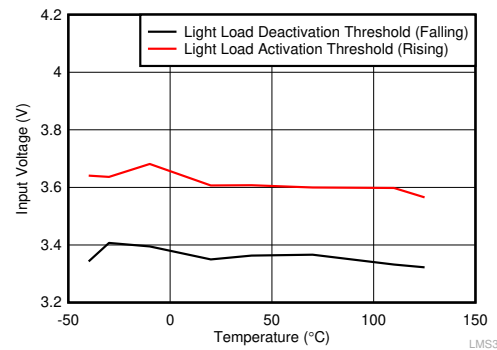
图 8-8. Input Voltage for Mode Change — 3.3-V Output, 10-μH Inductor
