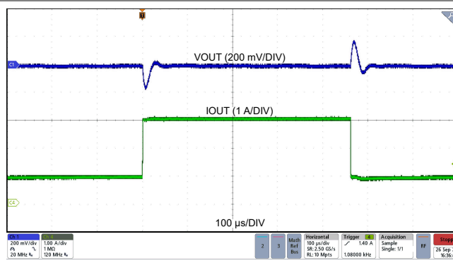
LMR66430R5R V_{OUT} = 5V 400kHz (自动) 1A 至 3A, 1A/ \mu s 修复
