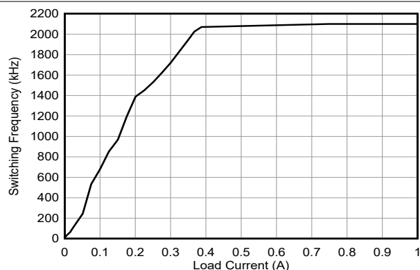
V IN = 12V 5V 输出 模式 = AUTO F sw = 2MHz
