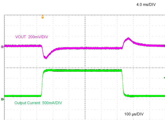
LMR38015 V_{OUT} = 5V 400kHz (交流耦合)
