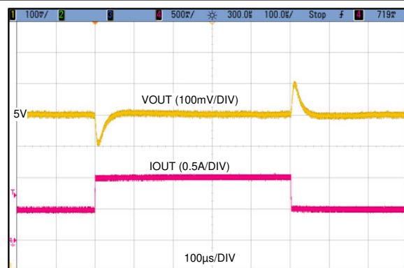
V_{OUT} = 5V 400kHz I_{LOAD} = 0.5A - 1A 压摆率 = 1 A/ \mu s
