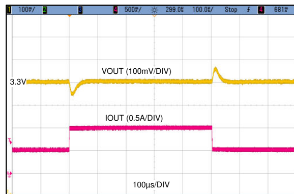
V_{OUT} = 3.3V 400kHz I_{LOAD} = 0.5A - 1A 压摆率 = 1 A/ \mu s
