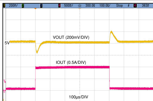
V_{OUT} = 5V 400kHz I_{LOAD} = 0.1A - 1A 压摆率 = 1 A/ \mu s
