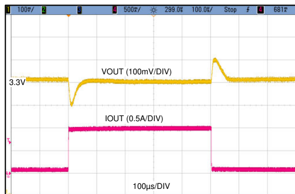
V_{OUT} = 3.3V 400kHz I_{LOAD} = 0.1A - 1A 压摆率 = 1 A/ \mu s
