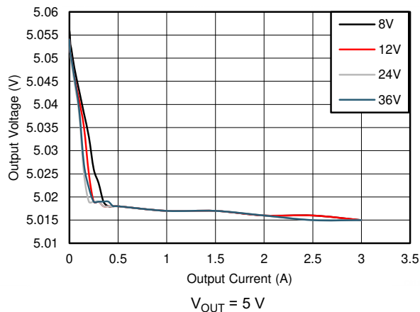
图 9-9. Line and Load Regulation
