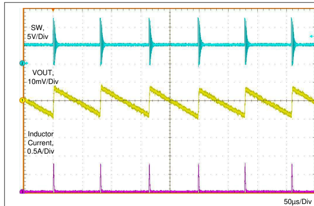
图 8-7. Typical PFM Switching Waveforms V_{IN} = 12 V, V_{OUT} = 5 V, I_{OUT} = 10 mA
