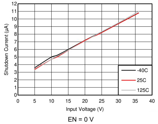
图 7-2. Shutdown Supply Current
