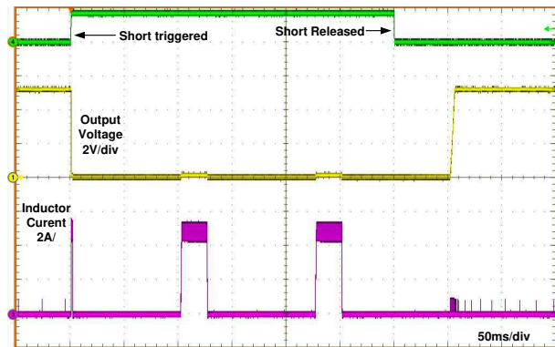
图 8-6. Short-Circuit Transient and Recovery
