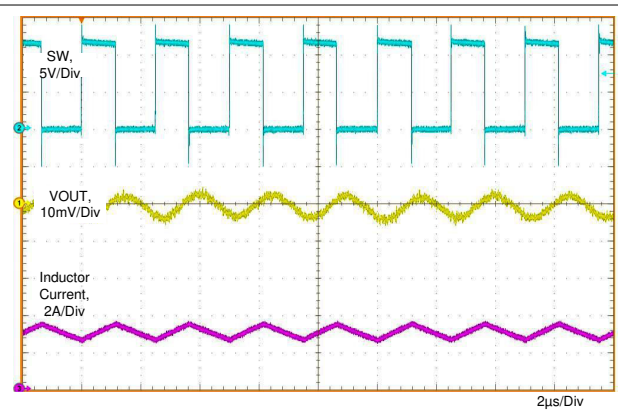
图 8-8. Typical PWM Switching Waveforms V_{IN} = 12 V, V_{OUT} = 5 V, I_{OUT} = 3 A, f_S = 400 kHz
