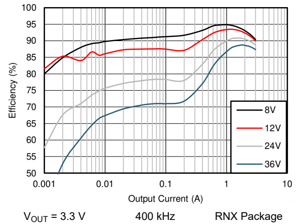
图 9-14. Efficiency
