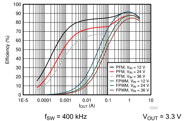
图 7-2. Efficiency vs Load Current
