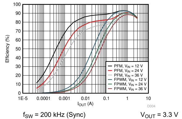
图 7-4. Efficiency vs Load Current
