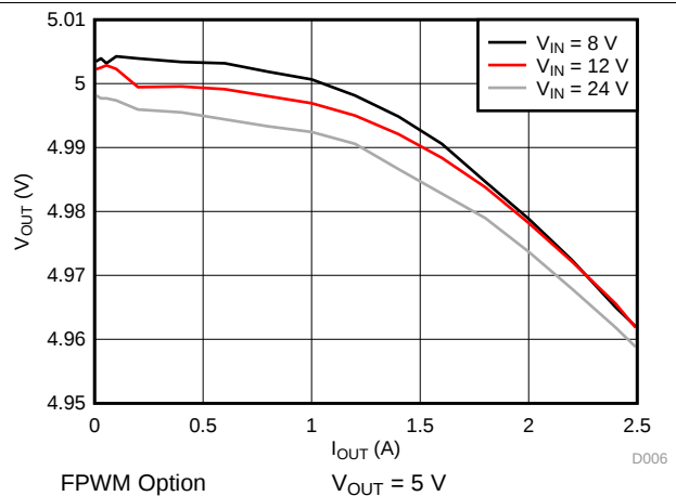
Figure 6. Load Regulation
