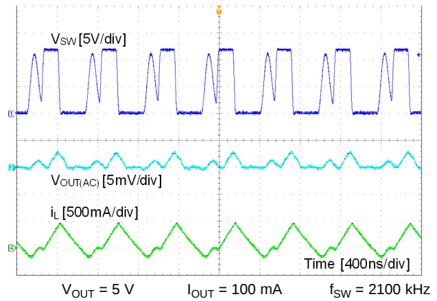
Figure 24. DCM Mode
