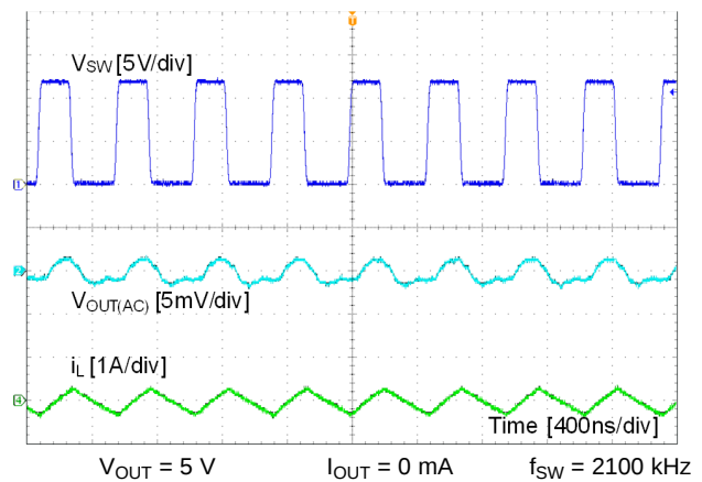
Figure 26. FPWM Mode
