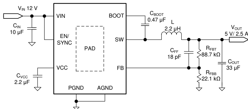
图 8-1. Application Circuit
