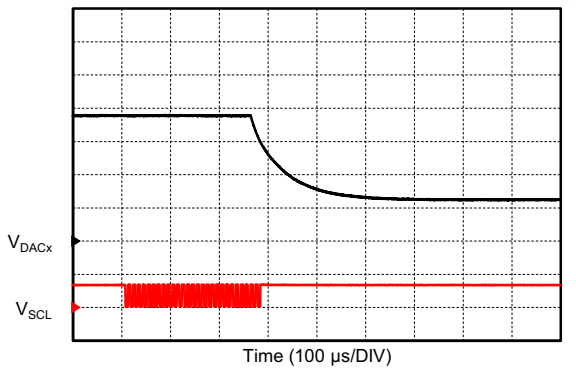
DAC OVERRIDE MODE C_L = 10\text{ }\mu\text{F} I^2\text{C} command triggers DAC step Step size: 3/4 to 1/4 FS
