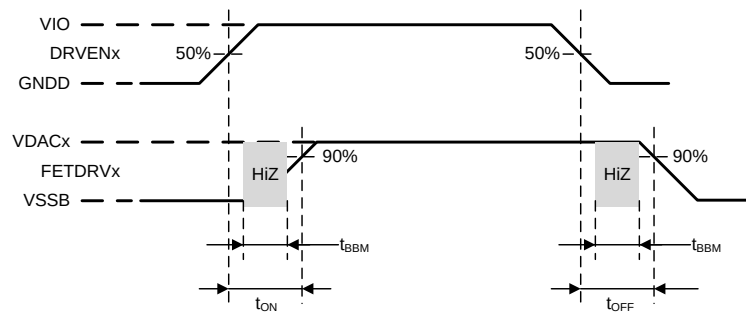
Figure 2. Switching
