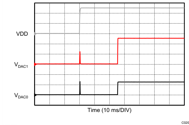
Figure 50. Power-Up Transient Behavior
