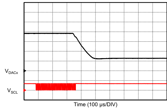
DAC OVERRIDE MODE C_L = 10\text{ pF} I^2\text{C} command triggers DAC step Step size: 3/4 to 1/4 FS
