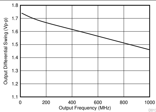
图 5-13. LVPECL Differential Output Swing vs Frequency
