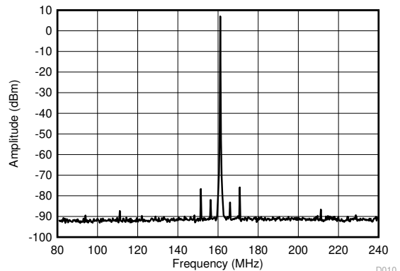
图 5-8. 156.25 ± 78.125MHz LVDS Differential Output Spectrum
