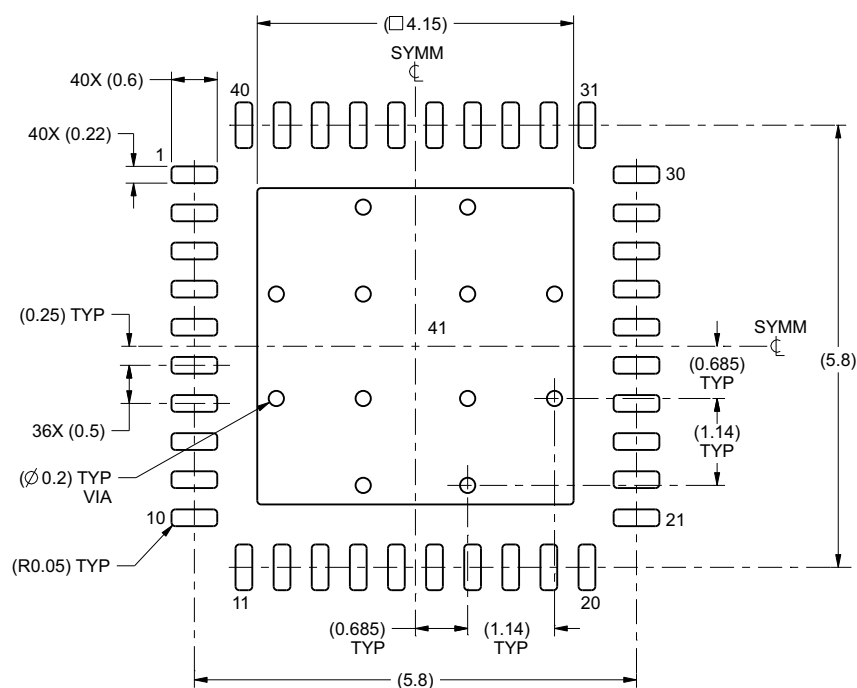
LAND PATTERN EXAMPLE SCALE:12X
