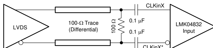
图 9-1. CLKinX/X* or OSCin Termination for an LVDS Reference Clock Source
