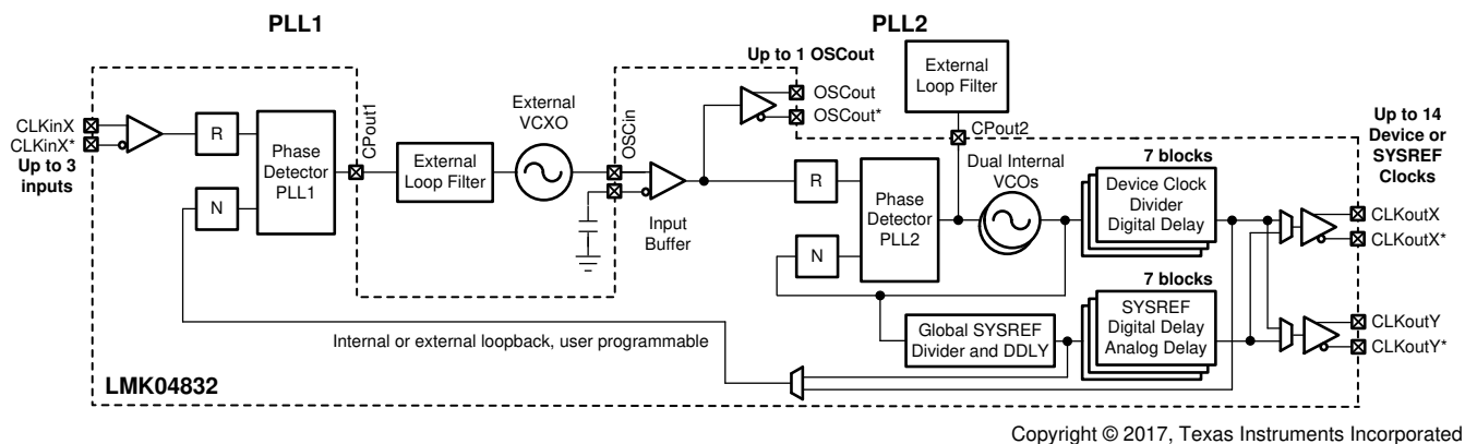
图 8-12. Simplified Functional Block Diagram for Nested 0-Delay Dual Loop Mode
