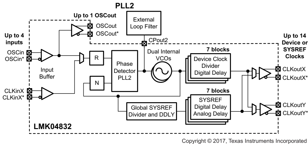
图 8-13. Simplified Functional Block Diagram for Single Loop Mode
