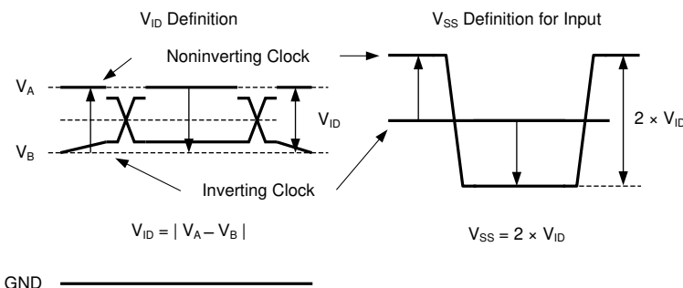
图 7-1. Two Different Definitions for Differential Input Signals
