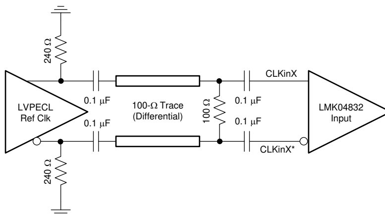
图 9-2. CLKinX/X* or OSCin Termination for an LVPECL Reference Clock Source
