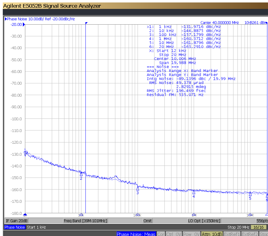
图 11. 40-MHz Input Phase Noise (181 fs rms, Light Blue), and Output Phase Noise (196 fs rms, Dark Blue), Additive Jitter = 77 fs rms
