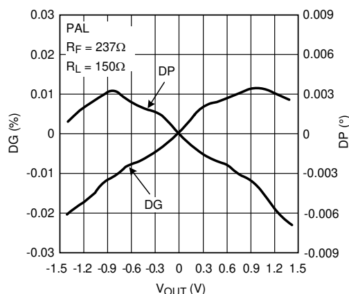
图 5-18. DG/DP (PAL)
