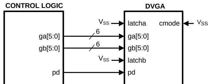
Figure 27. Parallel Mode Connection Not Using Latch Pins
