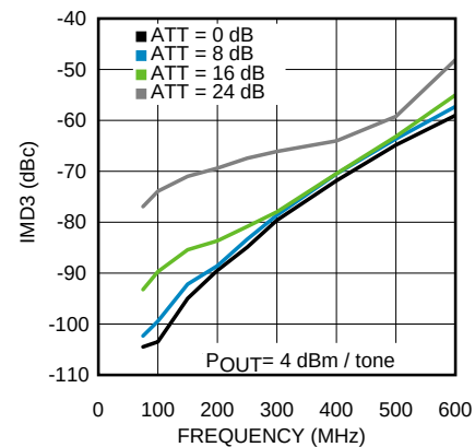
Figure 6. Third Order Intermodulation Products vs Frequency
