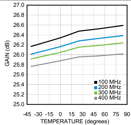
Figure 2. Gain Flatness vs Temperature
