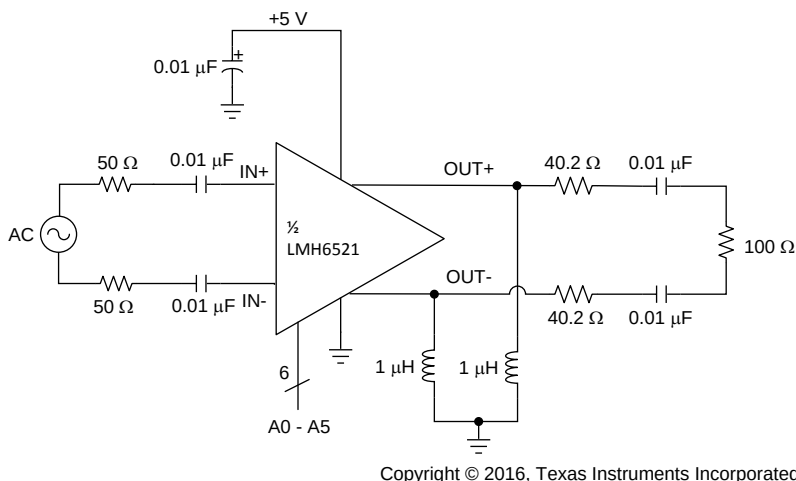
Figure 39. Basic Operating Connection
