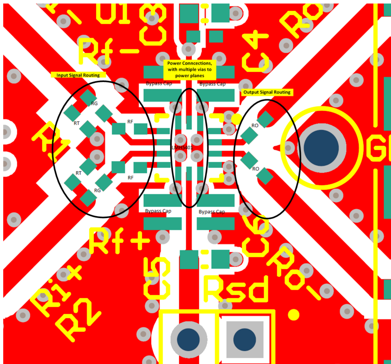
Figure 78. Layout Example
