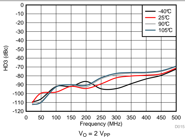
Figure 18. HD3 vs Frequency and Temperature
