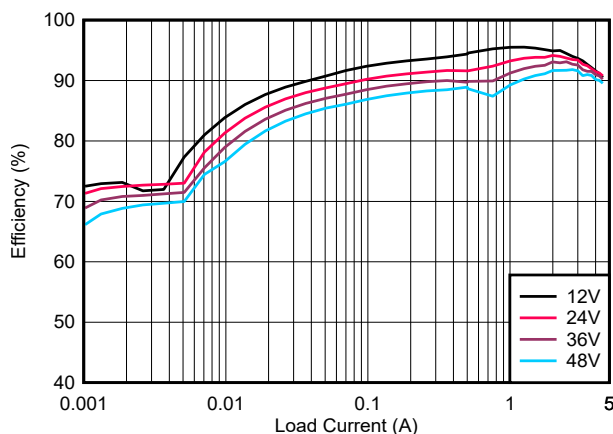
LM65645 效率, V_{OUT} = 5V , FSW = 400kHz
