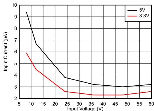
LM6x645 I_{OUT} = 0A L = 8.2 \mu H
