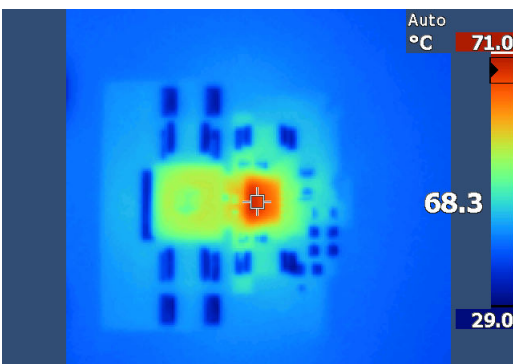
I_{OUT} = 6A 2100kHz V_{IN} = 12V V_{OUT} = 5V LM65460EVM
