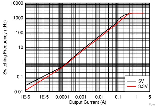
LM63625 V_{IN} = 13.5V F_{SW} = 2100kHz (自动)
