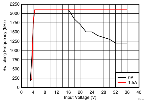
LM63615 V_{OUT} = 3.3V F_{SW} = 2100kHz (FPWM)
