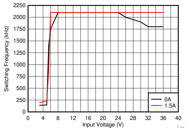
LM63615 V_{OUT} = 5V F_{SW} = 2100kHz (FPWM)
