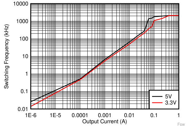
LM63615 V_{IN} = 13.5V F_{SW} = 2100kHz (自动)
