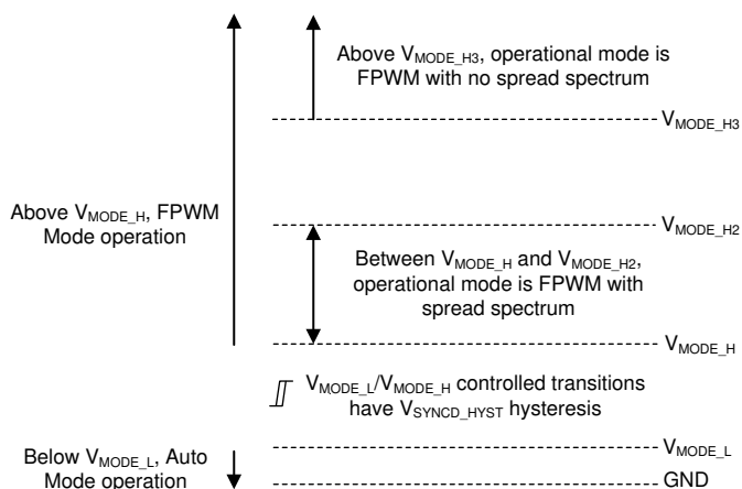
图 8-2. Level-Dependent Mode Selection Settings
