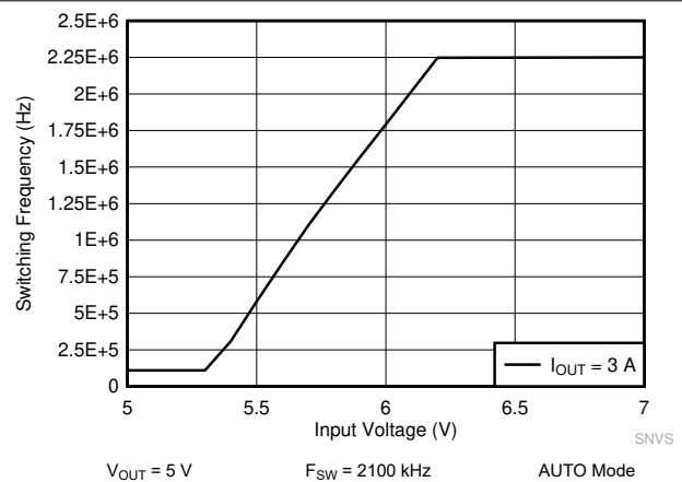
图 9-16. LM62435-Q1 Frequency Dropout Curve
