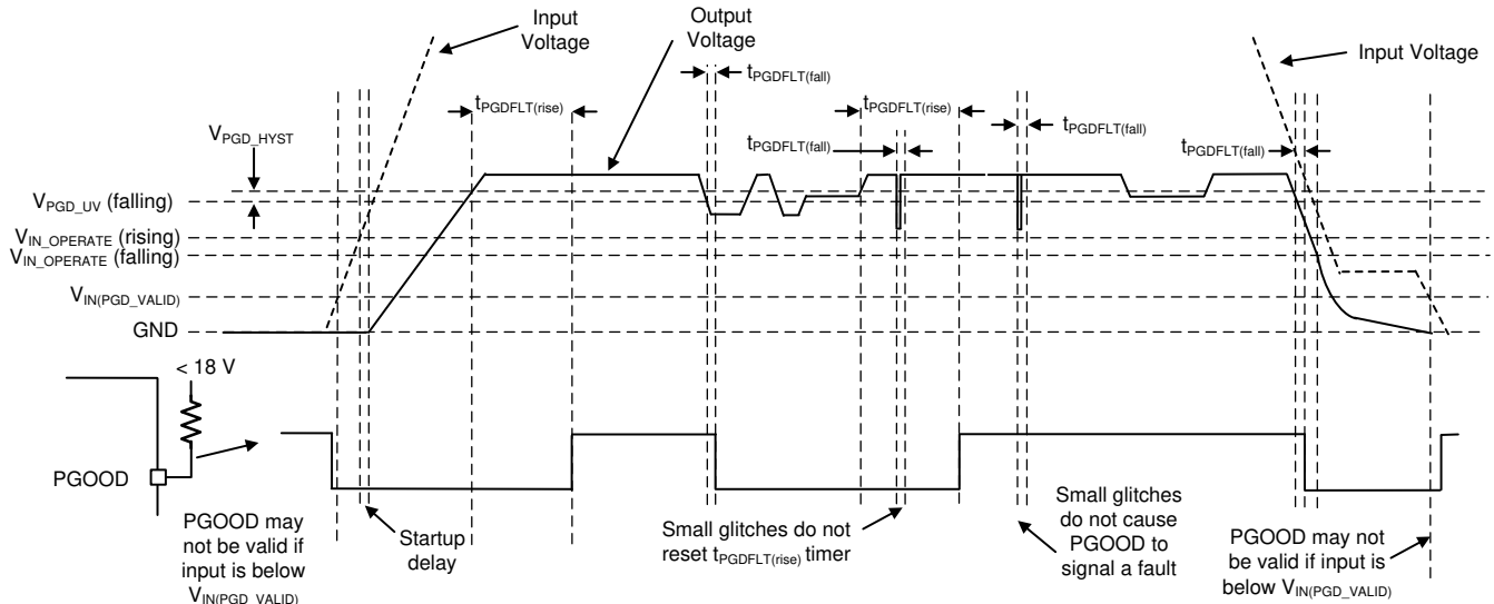
图 8-13. PGOOD Timing Diagram (Excludes OV Events)
