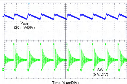
图 9-17. LM62435-Q1 Switching Waveform and V_{OUT} Ripple
