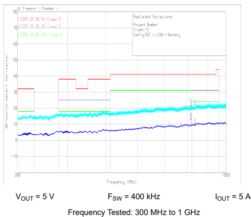
图 9-31. Radiated EMI Log Horizontal versus CISPR25 Limits
