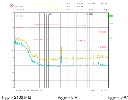
图 9-31. Radiated EMI Log Horizontal versus CISPR25 Limits
