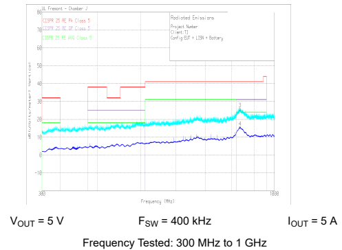
图 9-30. Radiated EMI Log Vertical versus CISPR25 Limits
