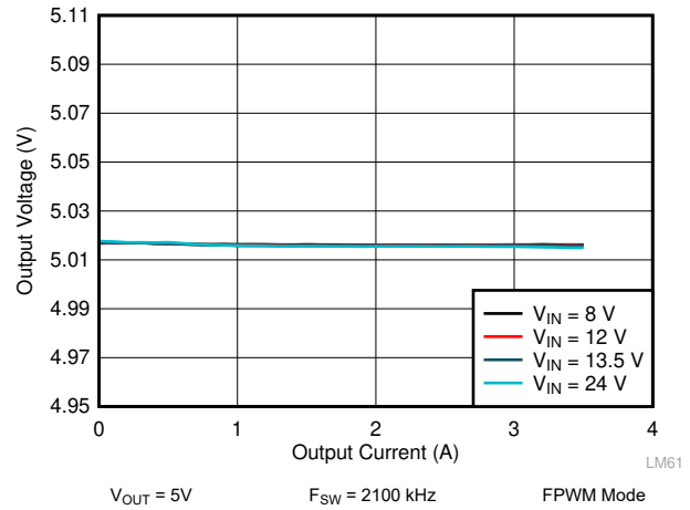
图 9-12. LM62435-Q1 Load and Line Regulation
