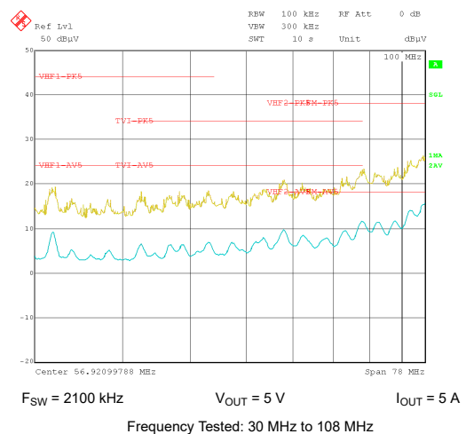
图 9-34. Conducted EMI versus CISPR25 Limits (Yellow: Peak Signal, Blue: Average Signal)
