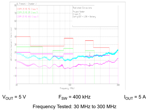
图 9-29. Radiated EMI Bicon Horizontal versus CISPR25 Limits
