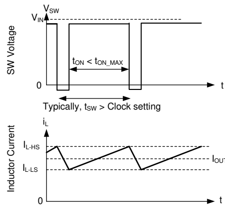
图 8-18. Current Limit Waveforms
