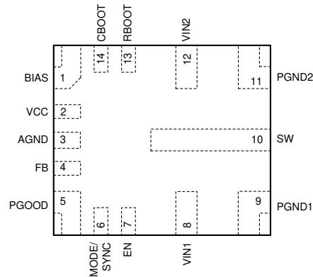
图 6-1. RJR Package 14-Pin VQFN-HR Top View
