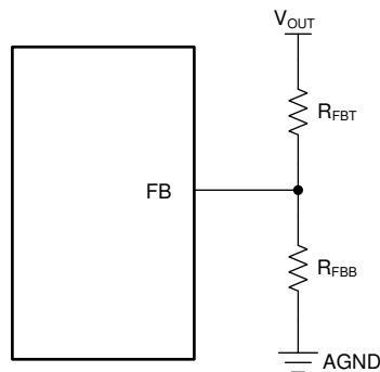
图 8-17. Setting Output Voltage of Adjustable Versions
