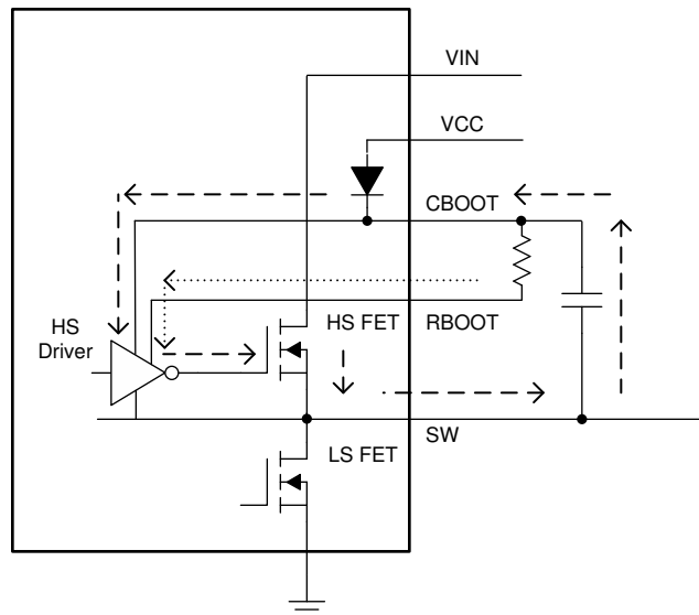
图 8-14. Simplified Circuit Showing How RBOOT Functions
