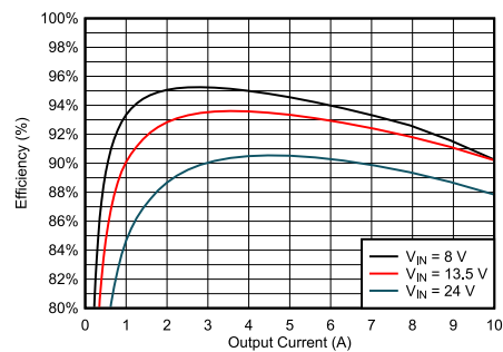
EVM 效率：，V OUT = 5V，F SW = 2.2 MHz
