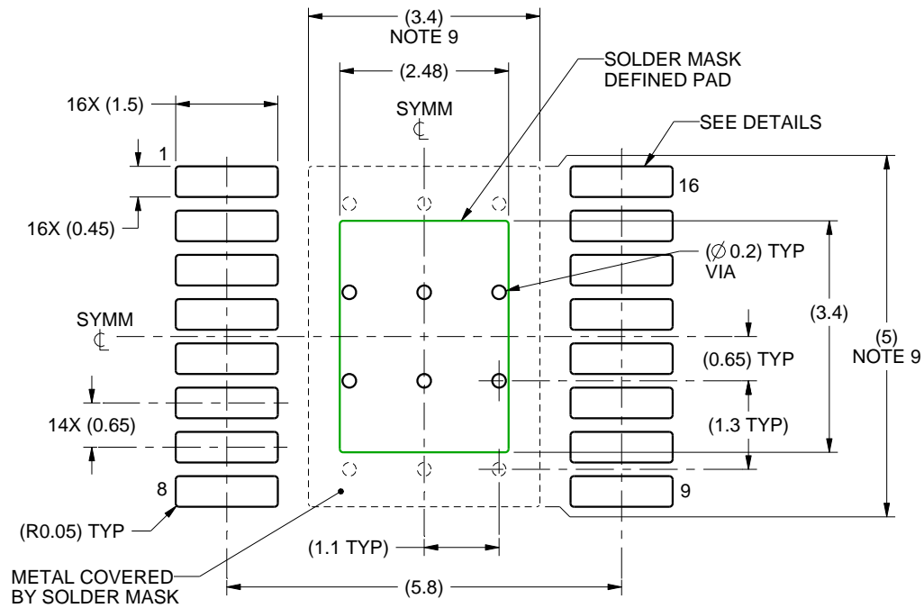
LAND PATTERN EXAMPLE SCALE:10X
