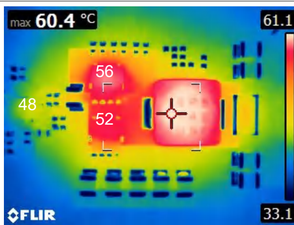
图 9-13. V_{\text{SUPPLY}} = 48\text{V} , I_{\text{LOAD}} = 8\text{A} , T_{\text{A}} = 25^{\circ}\text{C} , 无气流
