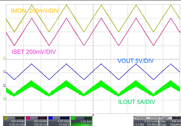
图 7-13. ISET 调制, V_{\text{SUPPLY}} = 48\text{V} , R_{\text{LOAD}} = 1.35\ \Omega
