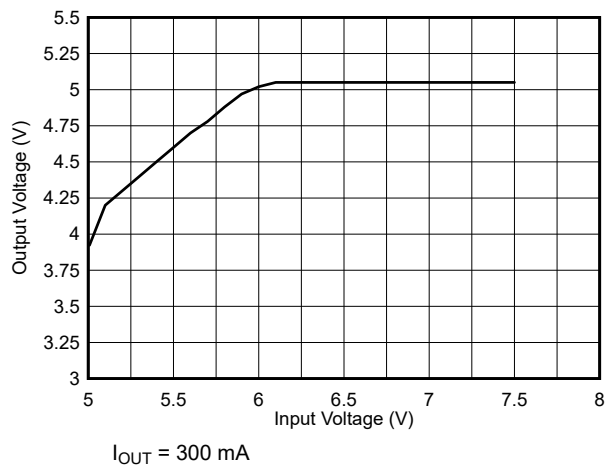
Figure 8-32. Drop-Out Response
