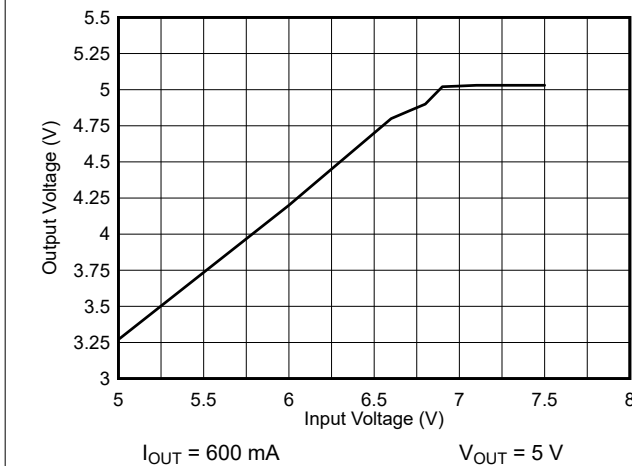
Figure 8-31. Drop-Out Response
