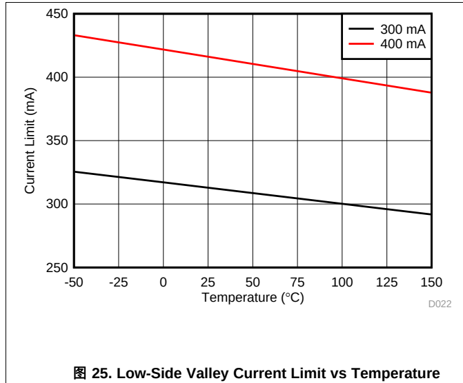
图 25. Low-Side Valley Current Limit vs Temperature
