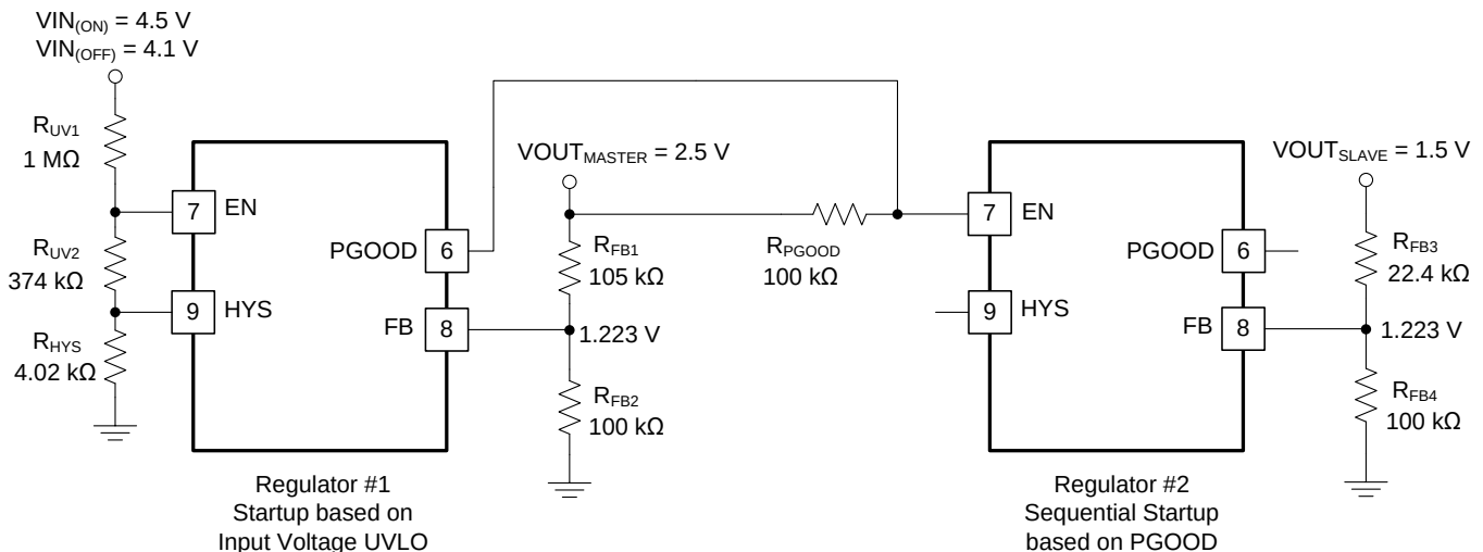
图 45. Master-Slave Sequencing Implementation Using PGOOD and EN
