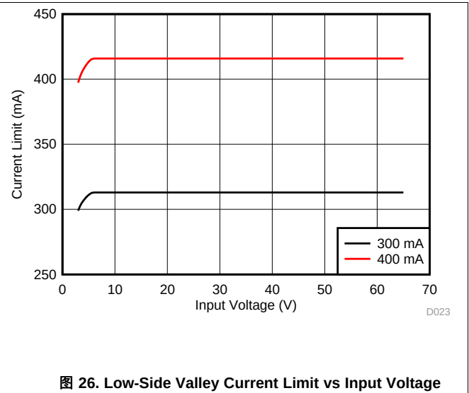
图 26. Low-Side Valley Current Limit vs Input Voltage
