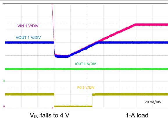
图 9-35. Cold-Crank Response to V_{IN} = 4 V
