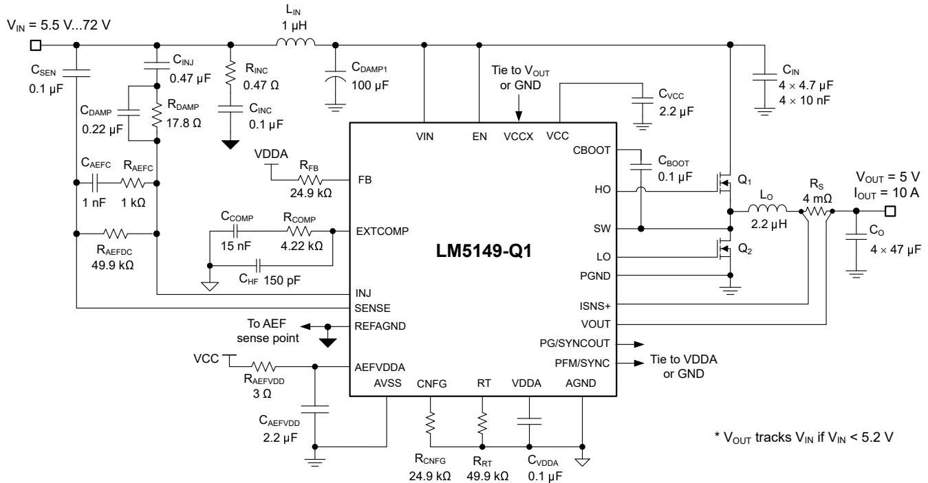
图 9-29. Application Circuit 3 With LM5149-Q1 Buck Regulator at 440 kHz
