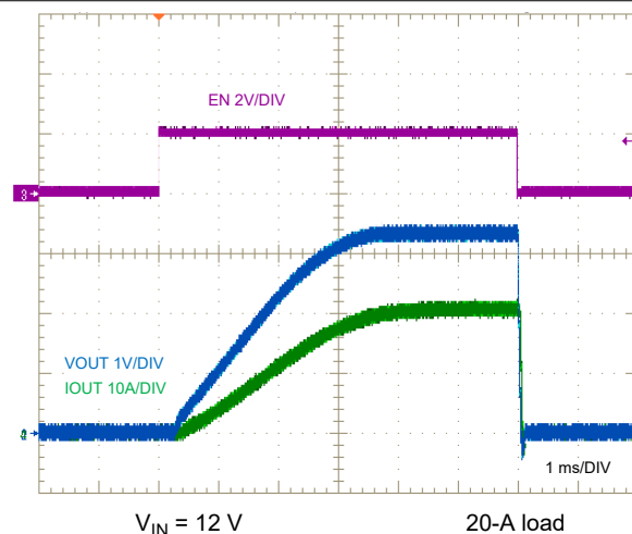
图 9-44. ENABLE ON and OFF Characteristic
