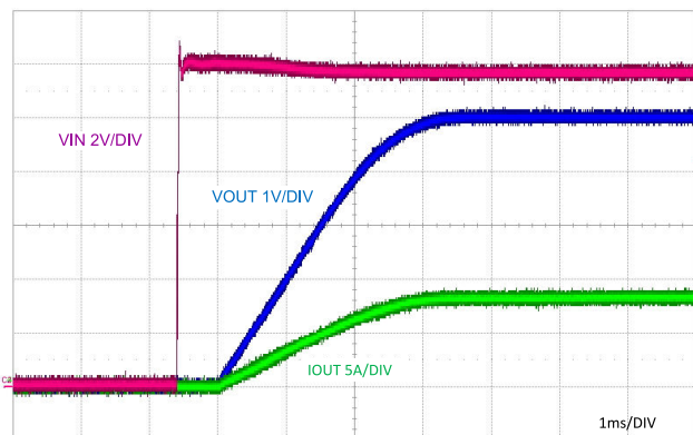
图 9-12. Start-Up Characteristic
