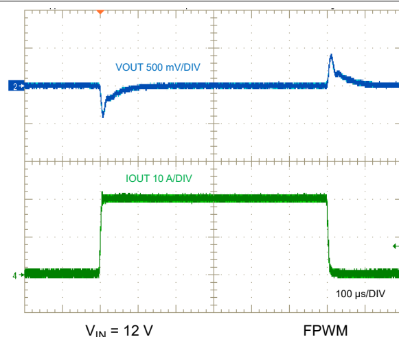
图 9-46. Load Transient, 0 A to 20 A
