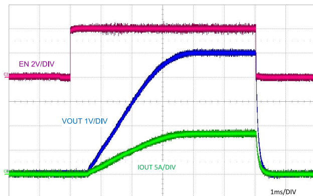
图 9-13. ENABLE ON and OFF Characteristic
