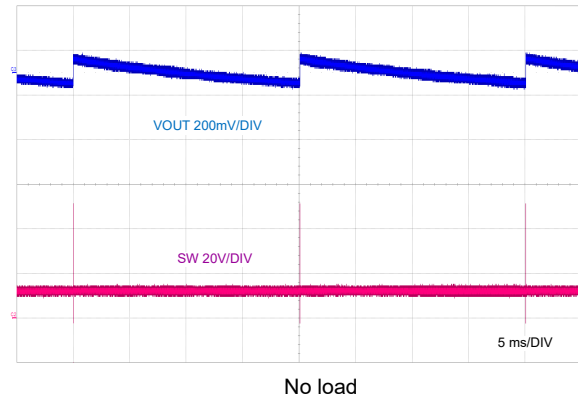
Figure 8-21. PFM Switching
