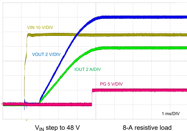
Figure 8-22. Start-Up Characteristic
