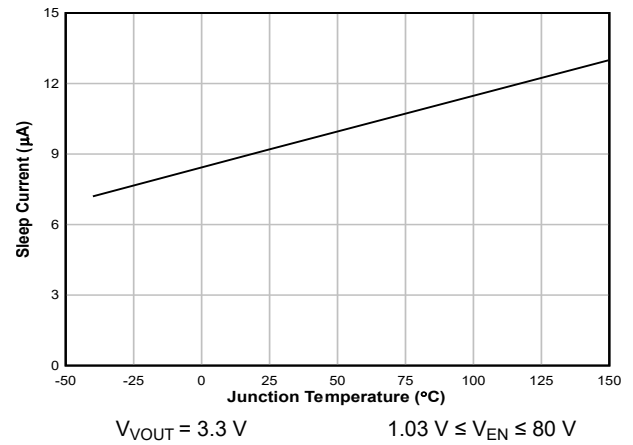
Figure 6-4. Sleep1 Current vs Temperature
