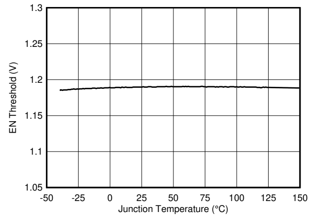
图 7-16. EN/UVLO Threshold vs Junction Temperature
