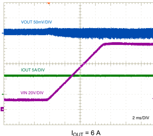
图 9-13. Line Transient Response, 12 V to 85 V
