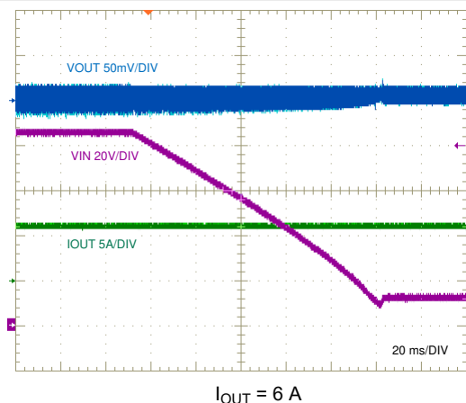
图 9-14. Line Transient Response, 85 V to 12 V
