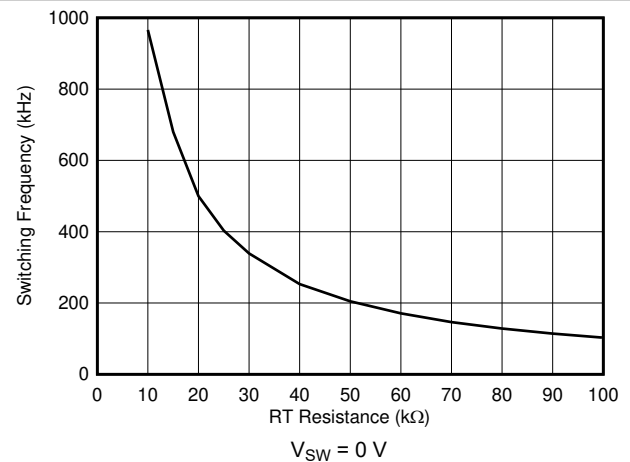
图 7-18. Oscillator Frequency vs RT Resistance
