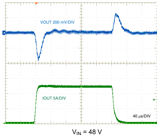
图 9-12. Load Transient Response, 0 A to 12 A to 0 A
