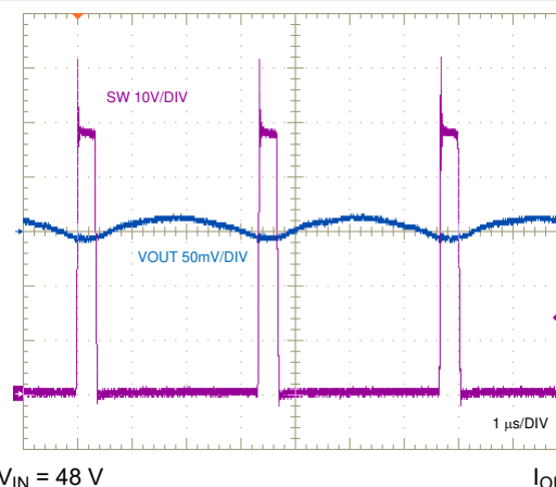
图 9-15. SW Node and Output Ripple Voltages
