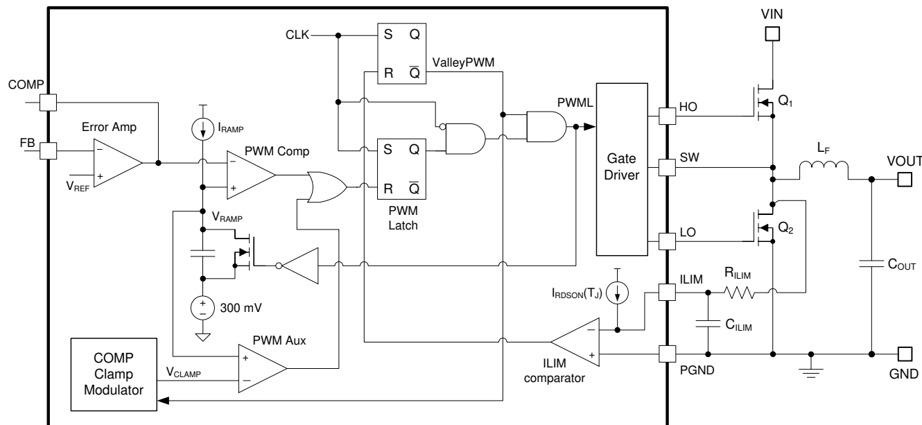
图 8-10. OCP Setpoint Defined by Current Source I_{RDSON} and Resistor R_{ILIM} in R_{DS-ON} Mode
