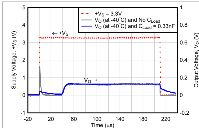
图 8-6. SR = 3.3V/\mu s 且无 C_{By-pass} 时, +V_S = 3.3V 阶跃的启动响应 (无 C_{Load} 且 C_{Load} = 0.33nF )
