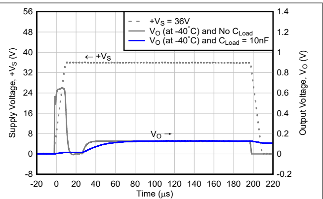
图 8-7. SR = 3.3V/\mu s 且无 C_{By-pass} 时, +V_S = 36V 阶跃的启动响应 (无 C_{Load} 且 C_{Load} = 10nF )
