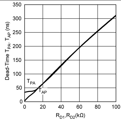
Figure 8. Dead-Time T_{PA} , T_{AP} vs. R_{D1} , R_{D2}
