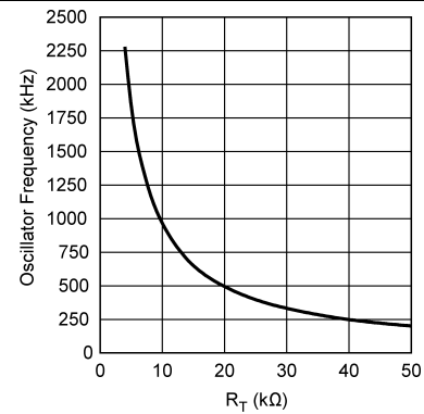
Figure 6. Oscillator Frequency vs. R_T
